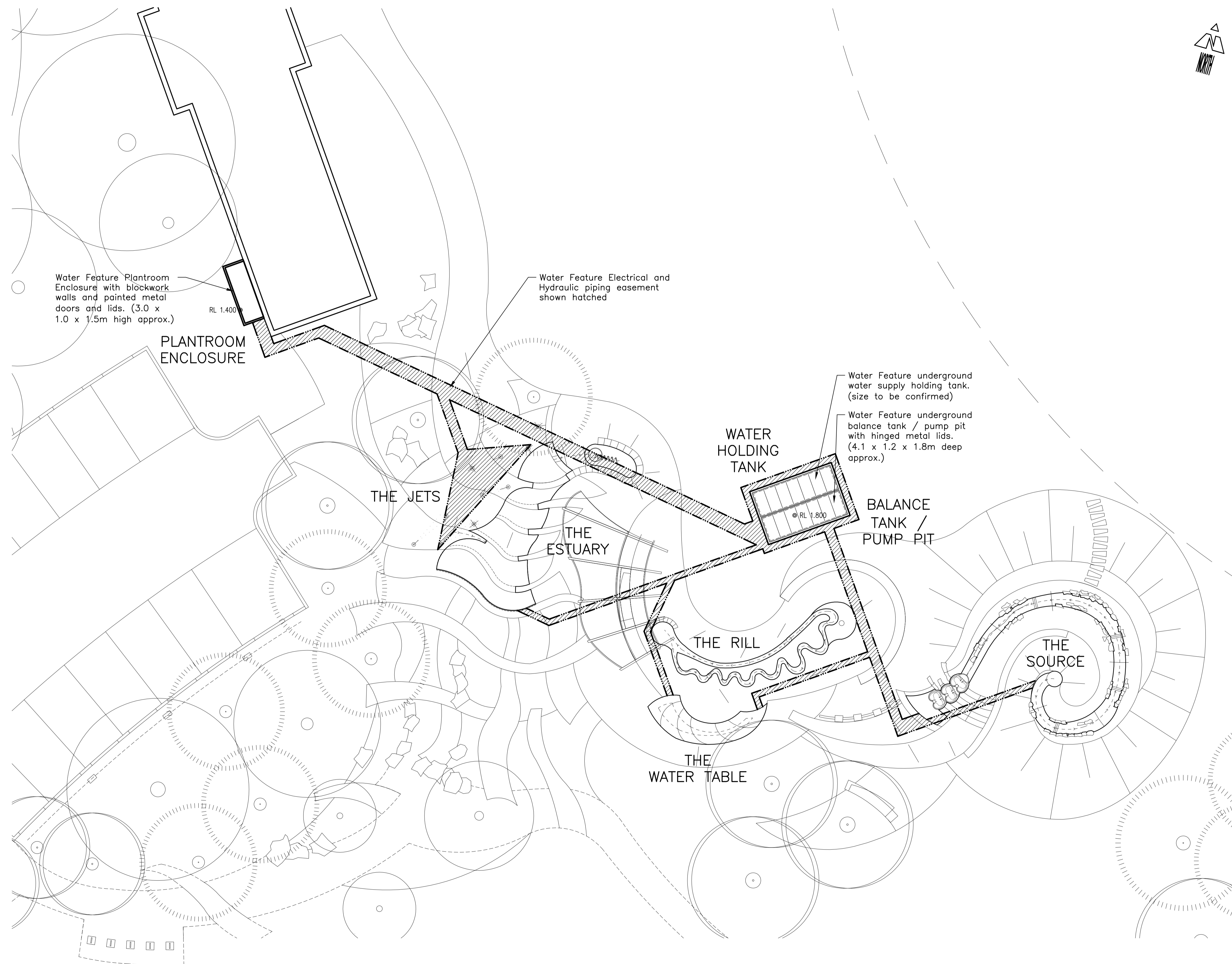
A PLAN – Water Feature Hydraulic Layout 1:100
